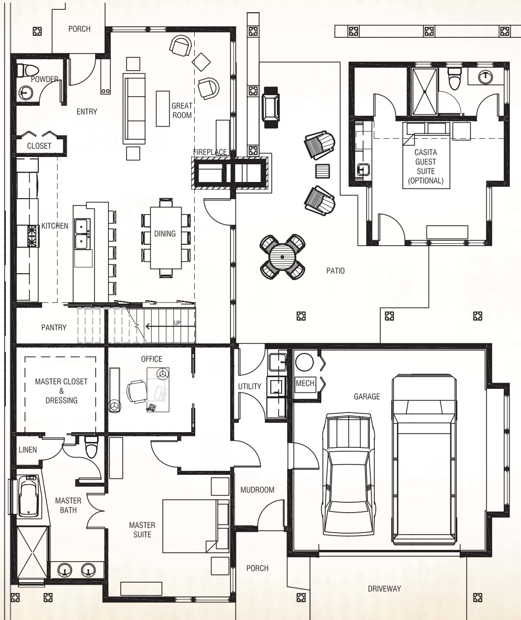
MAIN FLOOR PLAN (See other side for Upper Floor Plan) 3/32" = 1'-0"
