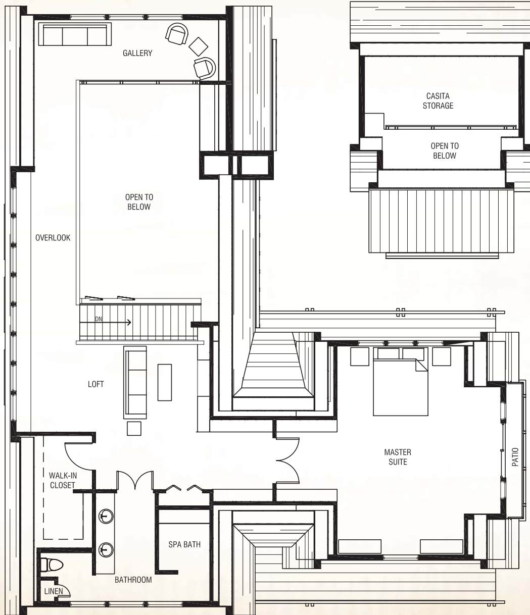
UPPER FLOOR PLAN (See other side for Main Floor Plan) 3/32" = 1'-0"
